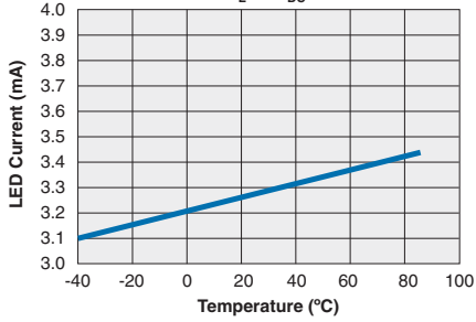
CPC1708 Typical I_F for Switch Operation vs. Temperature ( I_L=1A_{DC} )
