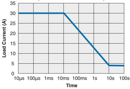
CPC1708 Energy Rating Curve (Free Air, No Heat Sink)
