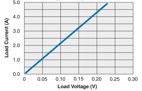
CPC1708 Typical Load Current vs. Load Voltage ( T_A=25°C, I_F=10mA )
