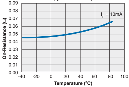
CPC1708 Typical On-Resistance vs. Temperature ( I_L=max\ rated )
