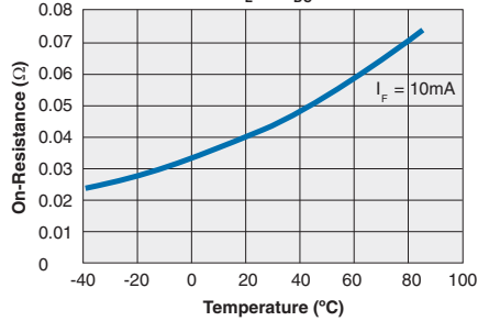
CPC1708 Typical On-Resistance vs. Temperature ( I_L=1A_{DC} )
